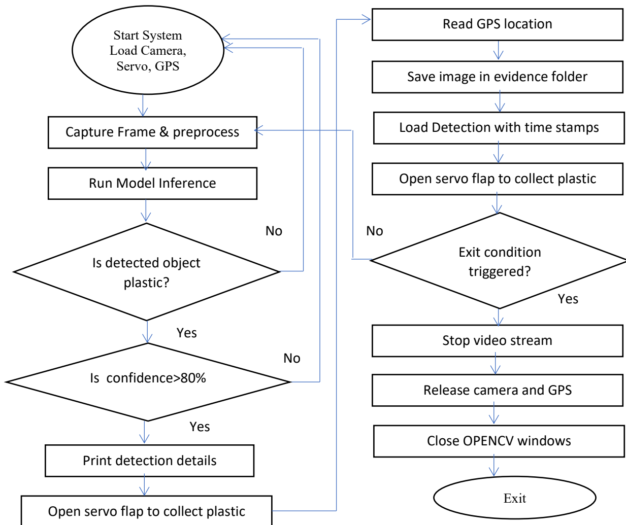
Figure 1: Process Flowchart
