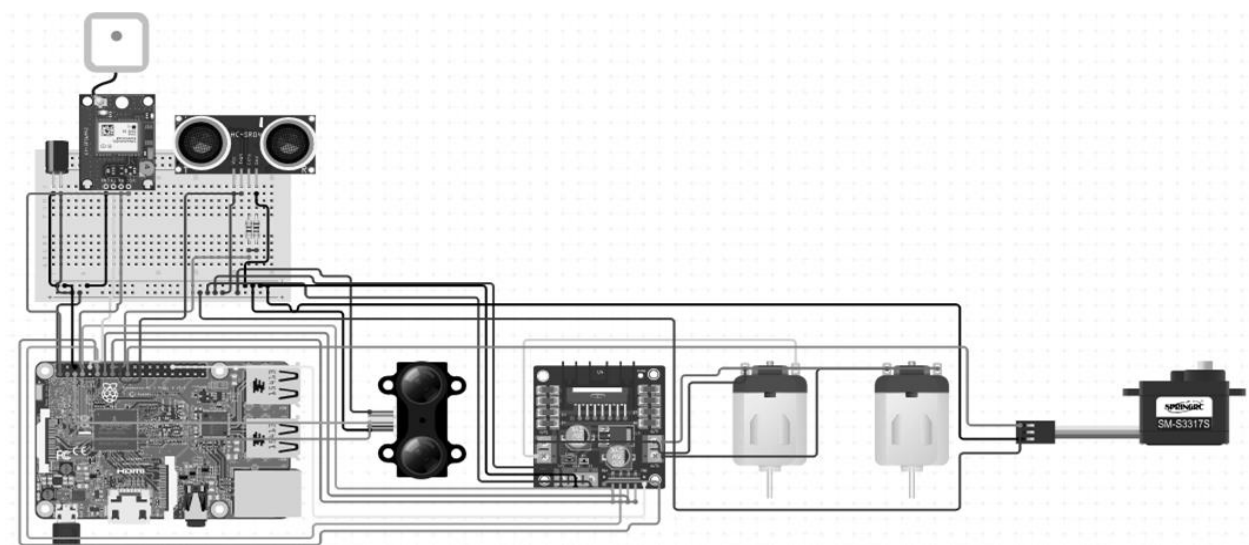
Figure 2 Connection Diagram
