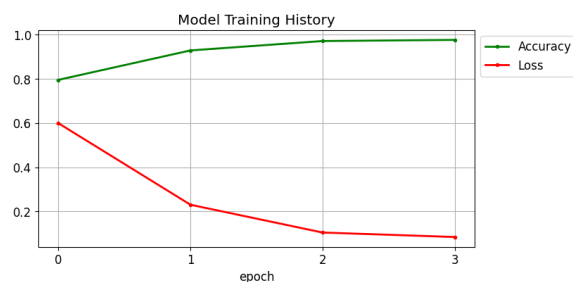
Figure 4.4. Model training information
