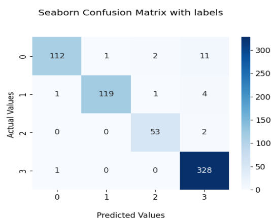
Figure 4.5 Confusion Matrix
