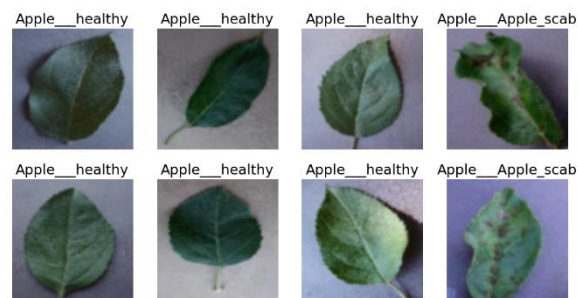
Figure 4.1: Input images
