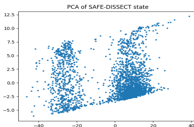
Fig. 2 Principal Component Analysis (PCA) State
