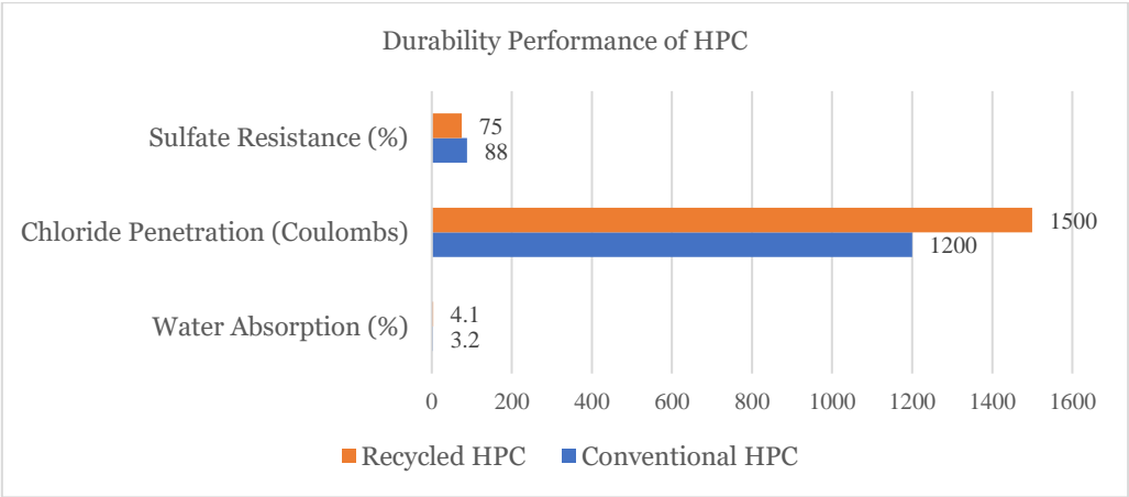
Figure 3: Durability Performance of HPC
