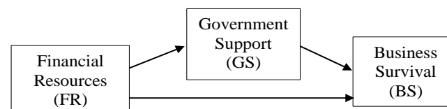
Figure 1. Research Model
