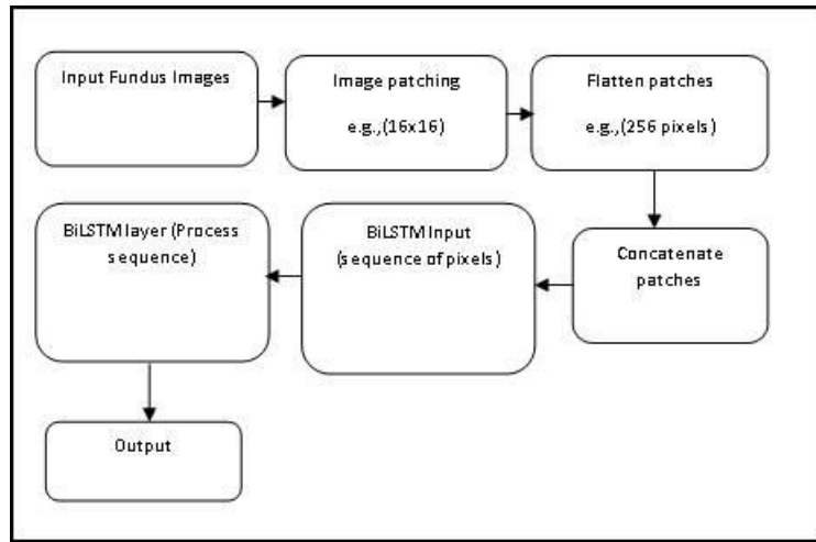
Fig.9. Input structure of BiLSTM
