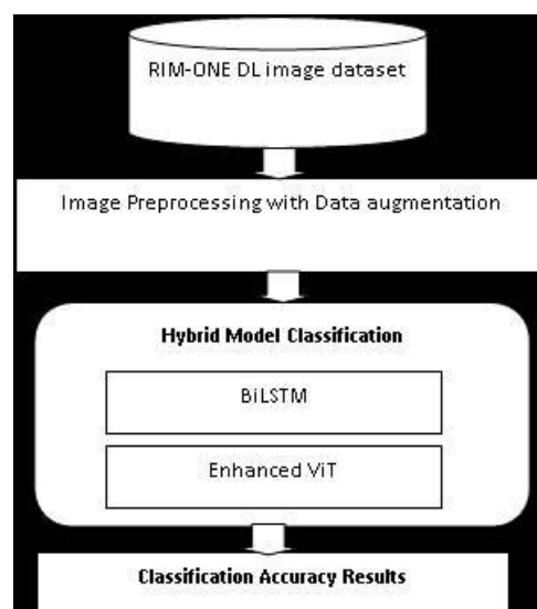
Fig.3. proposed Flow Diagram
