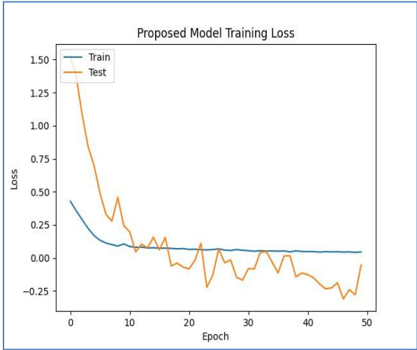
Fig.13. Proposed Hybrid Model Training and Validation Loss
