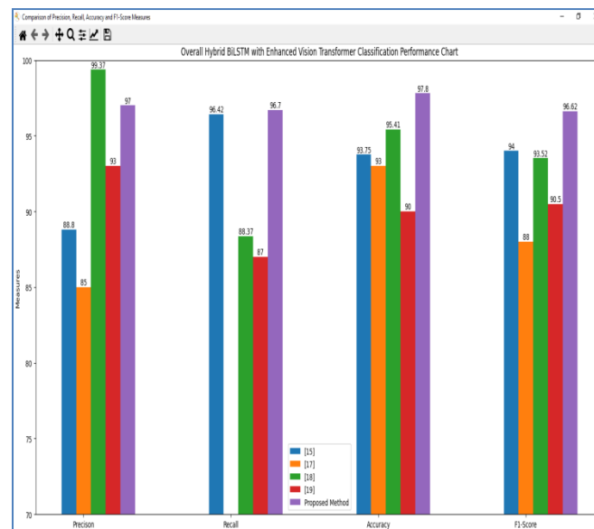
Fig. 14. Performance Analysis
