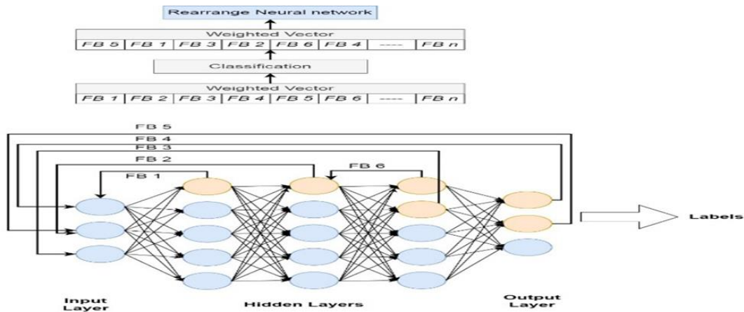
Figure 5: Design neural network
