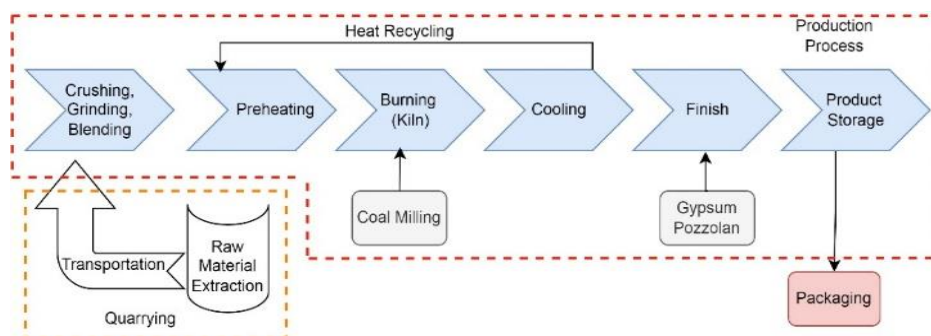
Fig 3: Cement Production Stages
