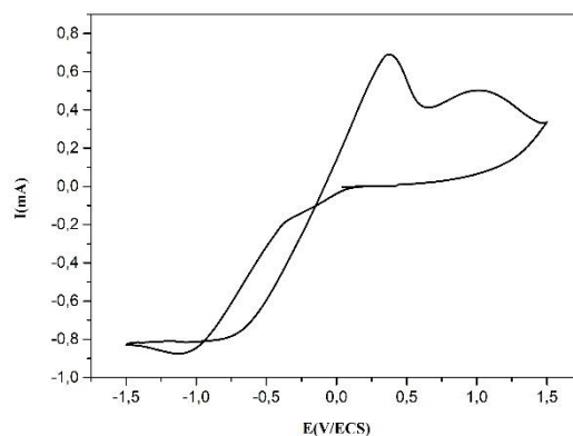
Figure 4: Cyclic voltammogram for a carbon black/PLA electrode in an aqueous solution of 10^{-1}\text{M} KCl and 10^{-2}\text{M} \text{CuCl}_2 at a scan rate of 50 mV/s; after pretreatment.
