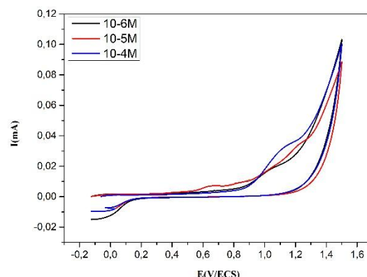
Figure 8: Oxidation curves of copper on a PLA printed electrode in an aqueous solution of 10^{-1}\text{M} KCl obtained at different concentrations of \text{CuCl}_2 : C_1=10^{-4}\text{M} , C_2=10^{-5}\text{M} and C_3=10^{-6}\text{M} , at v=50\text{mV/s} .
